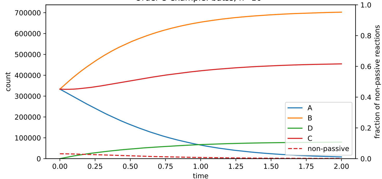
Order-3 example: batss, n=10^6
